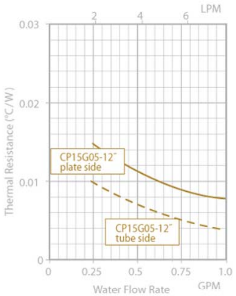
CP15G05 Thermal Resistance
