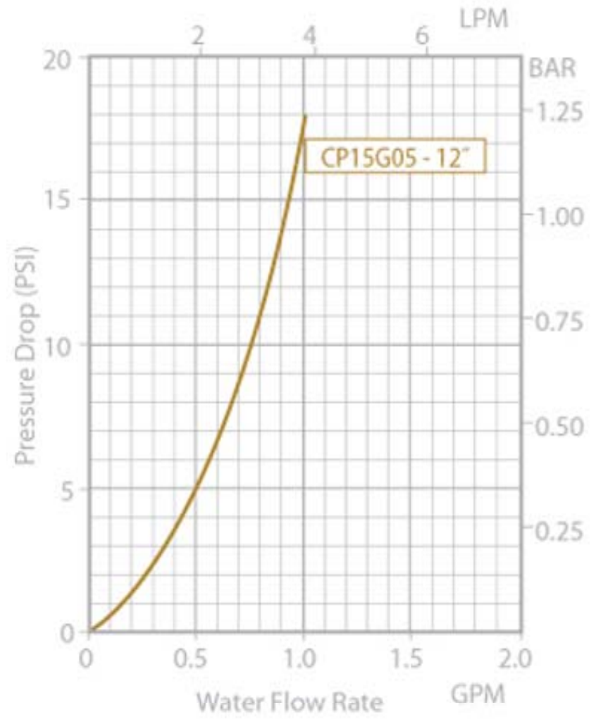
CP15G05 Pressure Drop
