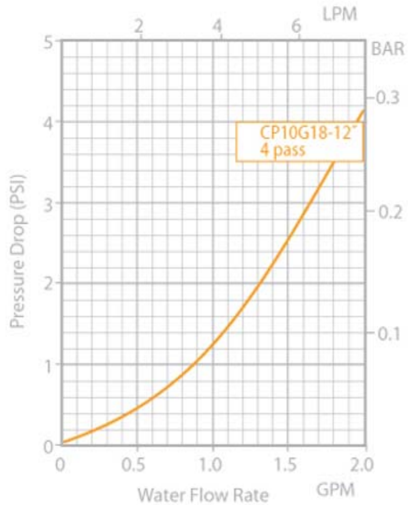
CP10G18 Pressure Drop
