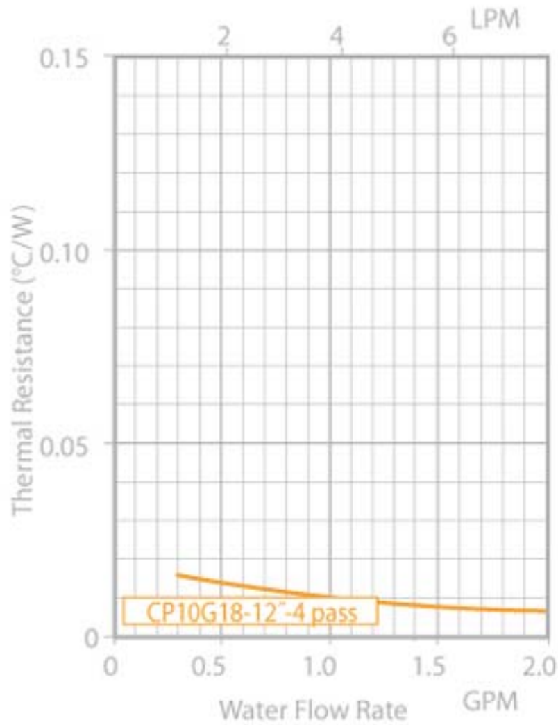
CP10G18 Thermal Resistance
