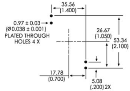
Mounting Details:
